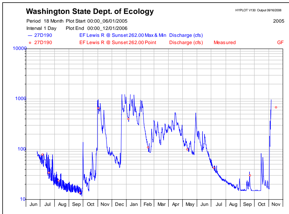
Figure 3: Discharge hydrograph for Site 2 June 1, 2005 – October 31, 2006.
