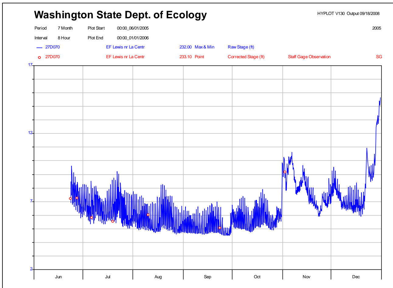
Figure 2. Tide-impacted stage height for Site 1, June 1 – December 31, 2005.
